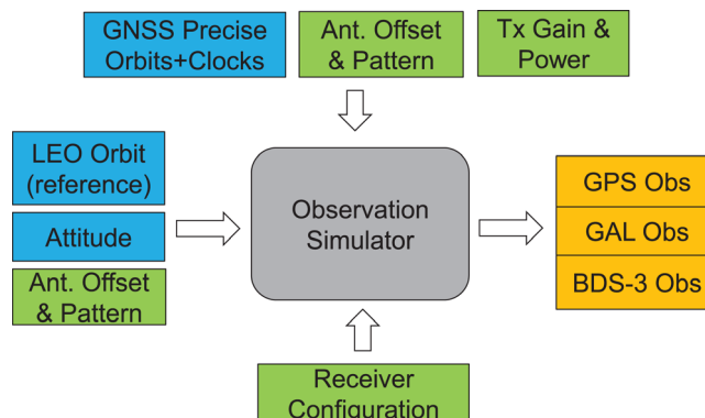
FIGURE 3 Simulation of multi-GNSS observations for spaceborne receivers. Individual colors indicate time varying motion and clock data (blue), static configuration parameters (green) and output data (orange) [Color figure can be viewed in the online issue, which is available at wileyonlinelibrary.com and www.ion.org ]
